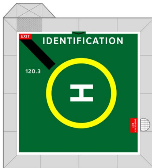
Figure 34: Unmanned facility Exit marking with Walkway marking
