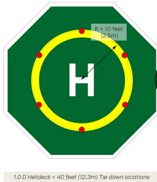
Figure 59: Tie-down point arrangement for 1.0D TLOF helideck with less than 40 ft. diameter
