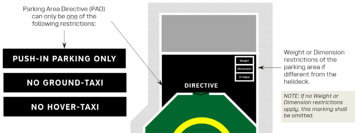
Figure 51: Parking Transition Area (PTA) associated markings
