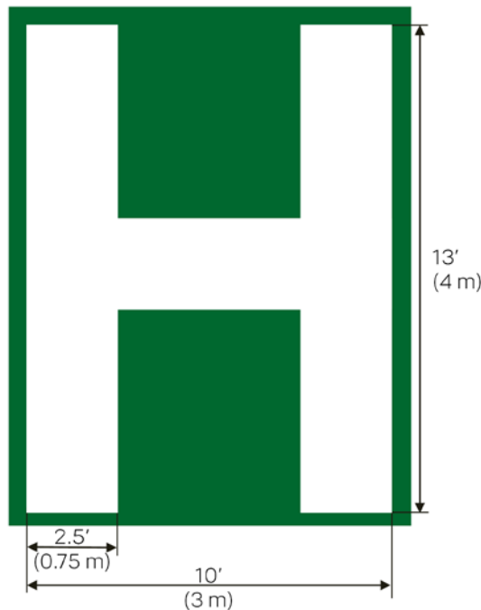
Figure 19: Helideck “H” marking
