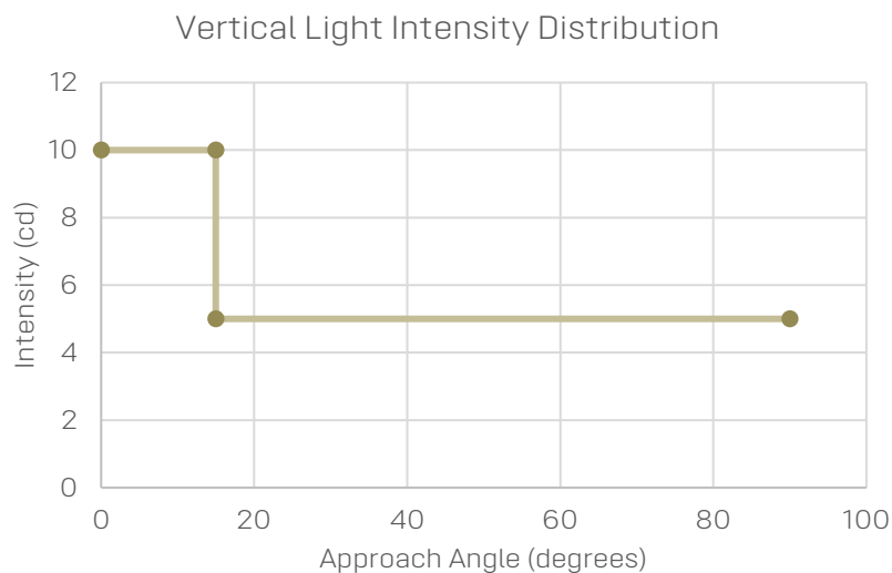
Figure 62: Vertical light intensity distribution
