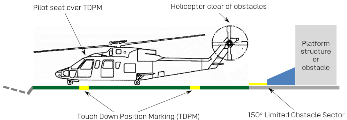
Figure 16: Relationship of the TDPM to LOS for a 1.0D TLOF
