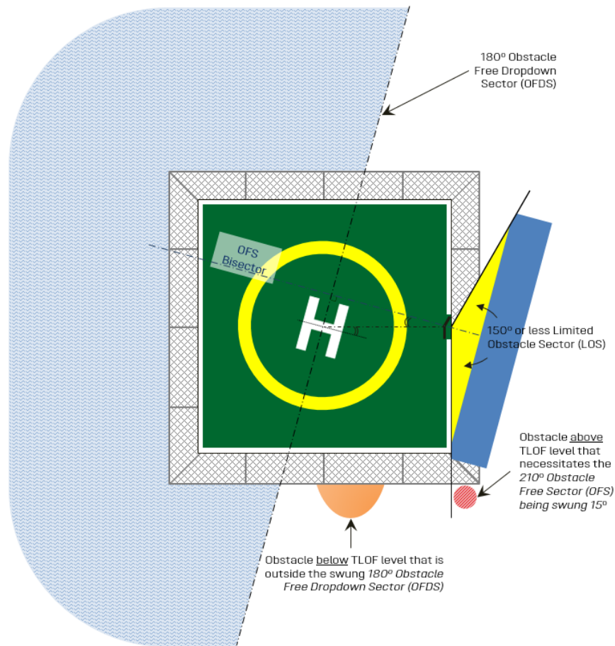
Figure 13: Obstacle Free Sector swung by 15 degrees
