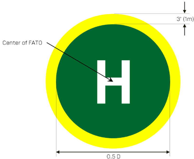
Figure 18: TDPM and "H" marking
