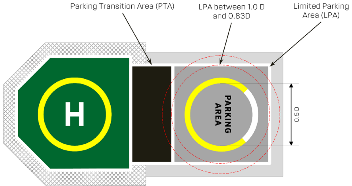
Figure 41: Limited Parking Area (LPA) of 0.83D with Parking Circle Orientation Marking (PCOM)
