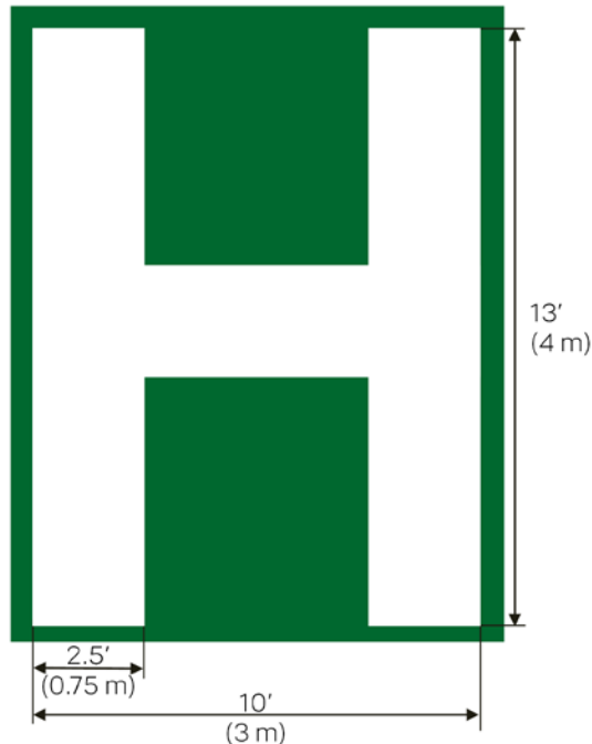
Figure 19: Helideck 'H' Marking
