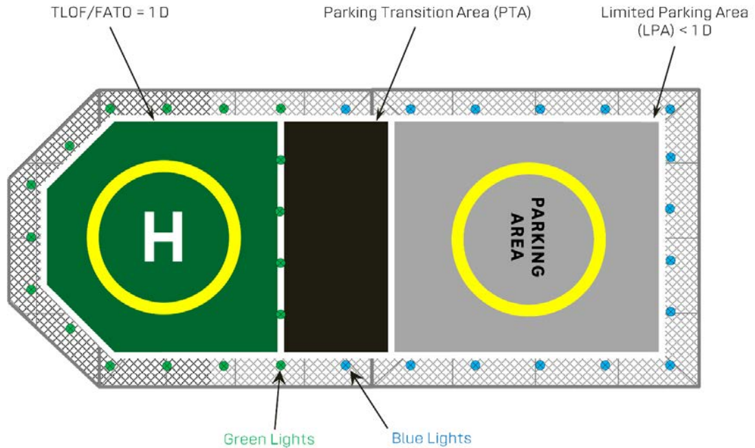
Figure 38: Parking Area lighting arrangement
