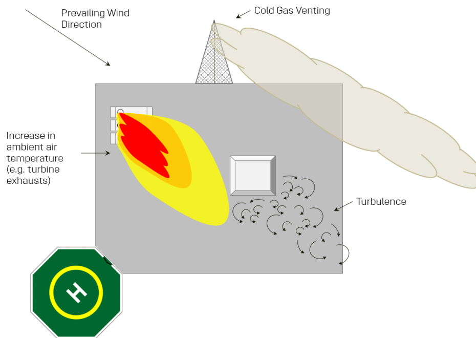
Figure 1: Helideck orientation based on wind direction, turbulence, and significant discharge sources
