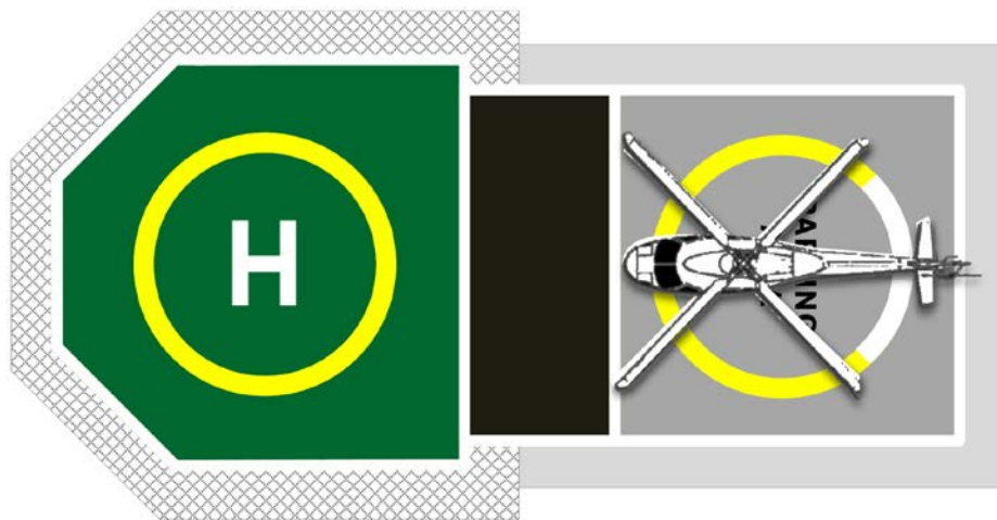
Figure 42: Helicopter parked using Parking Circle Orientation Marking (PCOM)
