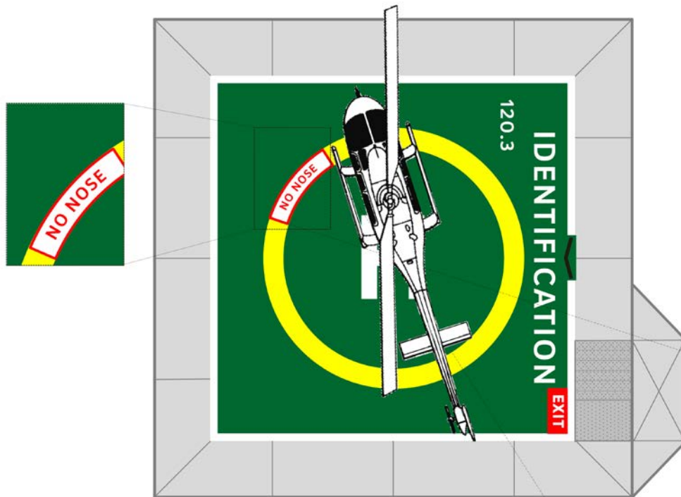
Figure 32: "No Nose" marking
