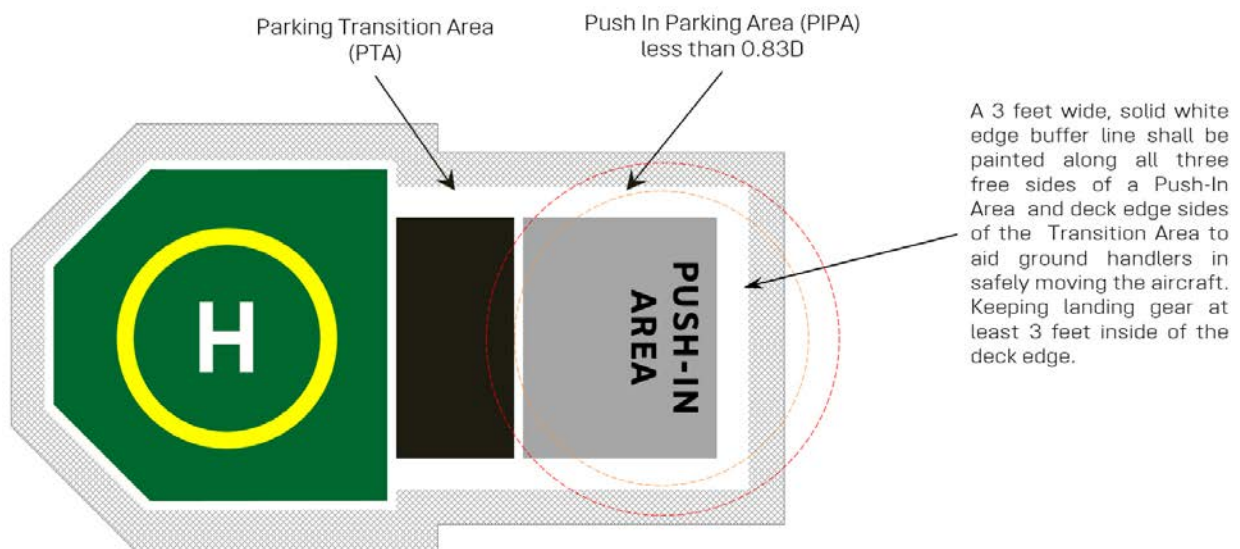
Figure 48: Push-In Parking Area (PIPA)
