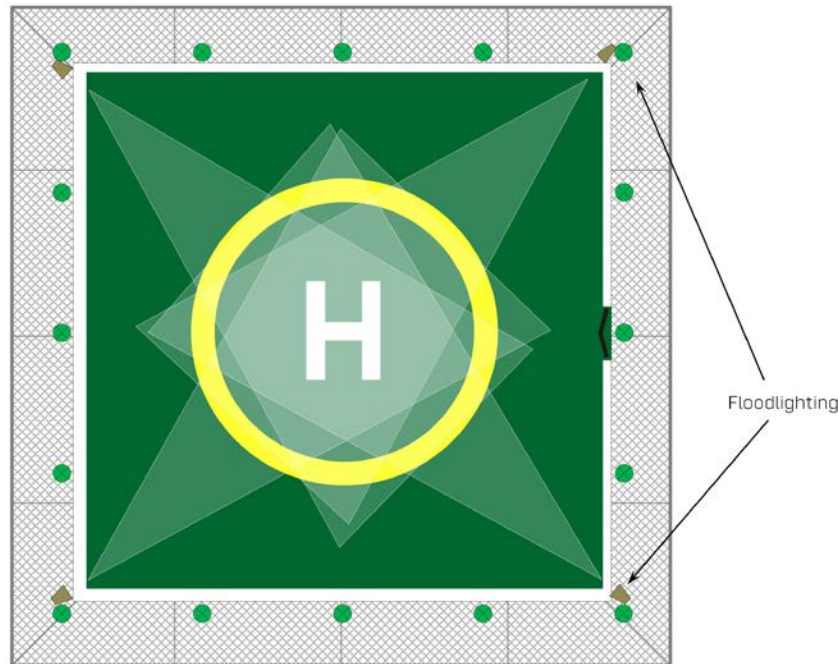
Figure 37: Typical Floodlighting arrangement
