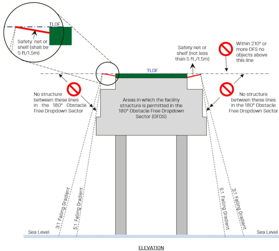
Figure 12: Obstacle Free Sector (OFS) and Obstacle Free Dropdown Sector (OFDS)
