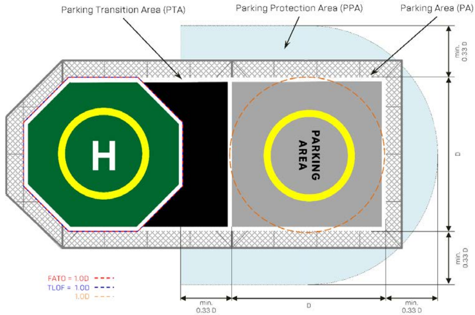
Figure 4: 1.0D FATO and 1.0D TLOF with a 1.0D Parking Area
