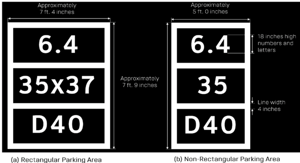
Figure 52: Parking Area size/weight markings (U.S. customary units)
