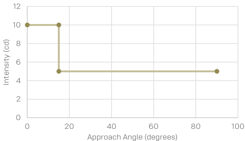
Vertical Light Intensity Distribution
