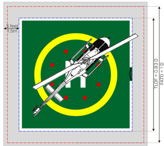
Figure 56: Tie-down point arrangement for an offshore-based helicopter on 0.83D TLOF helideck (b)
