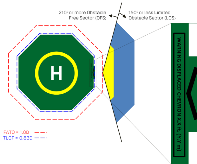
Figure 29: Displaced chevron marking
