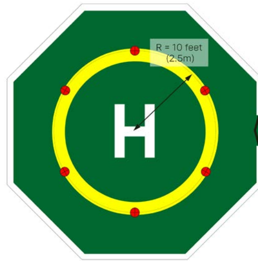
1.0 D Helideck < 40 feet (12.3m) Tie-down locations
