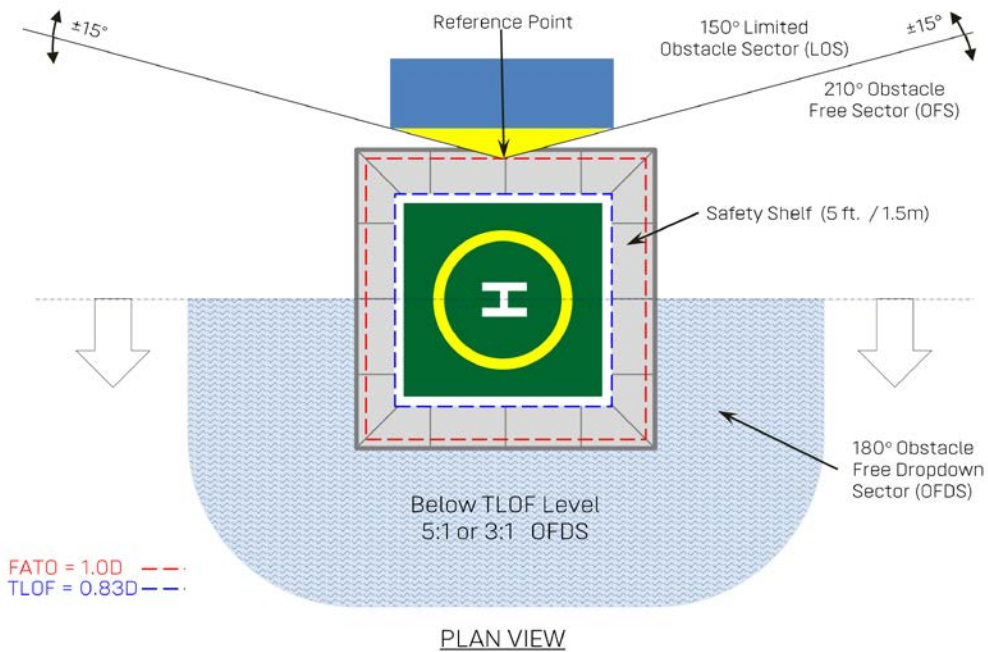
Figure 11: OFS, LOS, and OFDS below a helideck with 0.83D square TLOF
