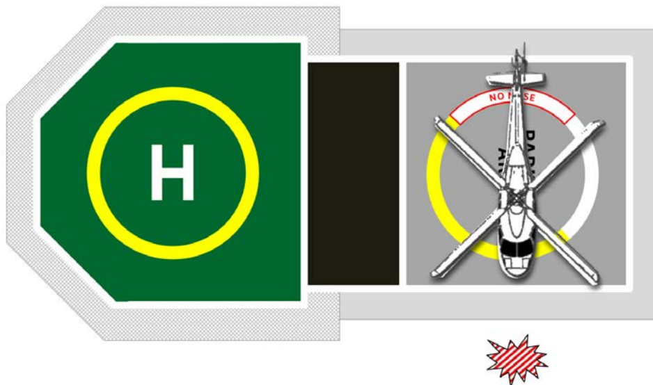
Figure 47: 'No Nose' marking and PCOM on TDPC with parked helicopter
