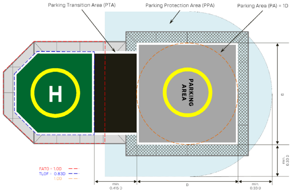
Figure 5: 1.0D FATO and 0.83D TLOF with a 1.0D Parking Area
