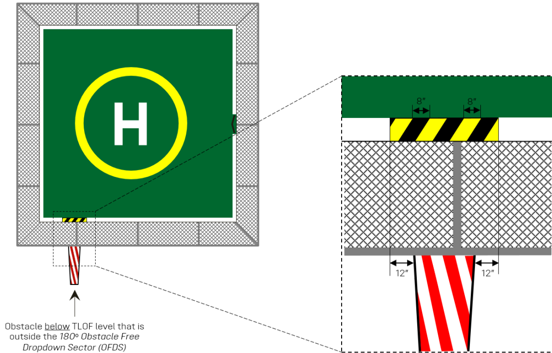
Figure 31: Obstacle Warning Marking for OFDS
