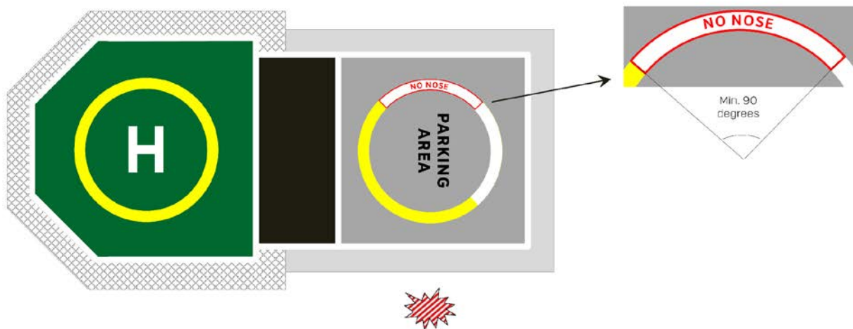
Figure 43: 'No Nose' marking and Parking Circle Orientation Marking (PCOM) on TDPC
