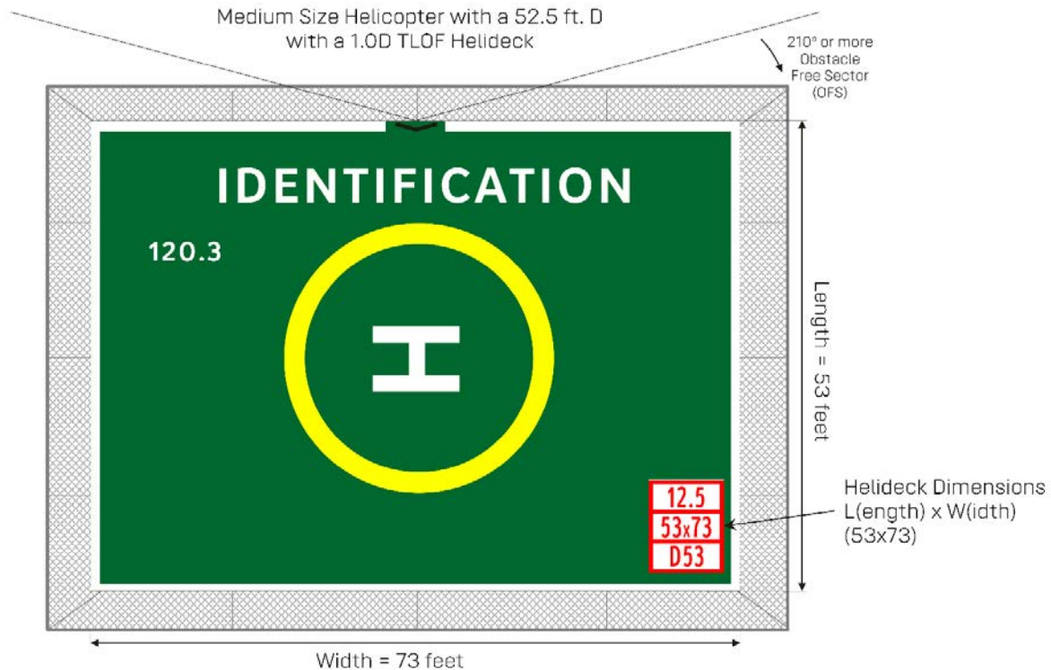
Figure 20: Size and weight markings for 1.0D 52.5 ft. medium helicopter rectangular helideck
