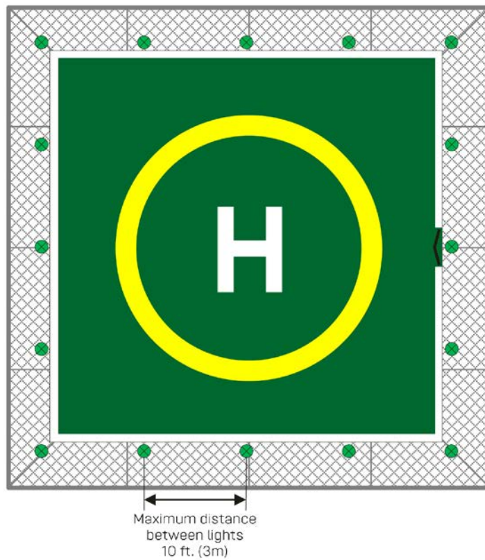
Figure 35: Square shaped TLOF helideck Perimeter Lighting arrangement
