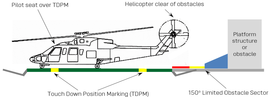
Figure 17: Relationship of the TDPM to LOS for a 0.83D TLOF
