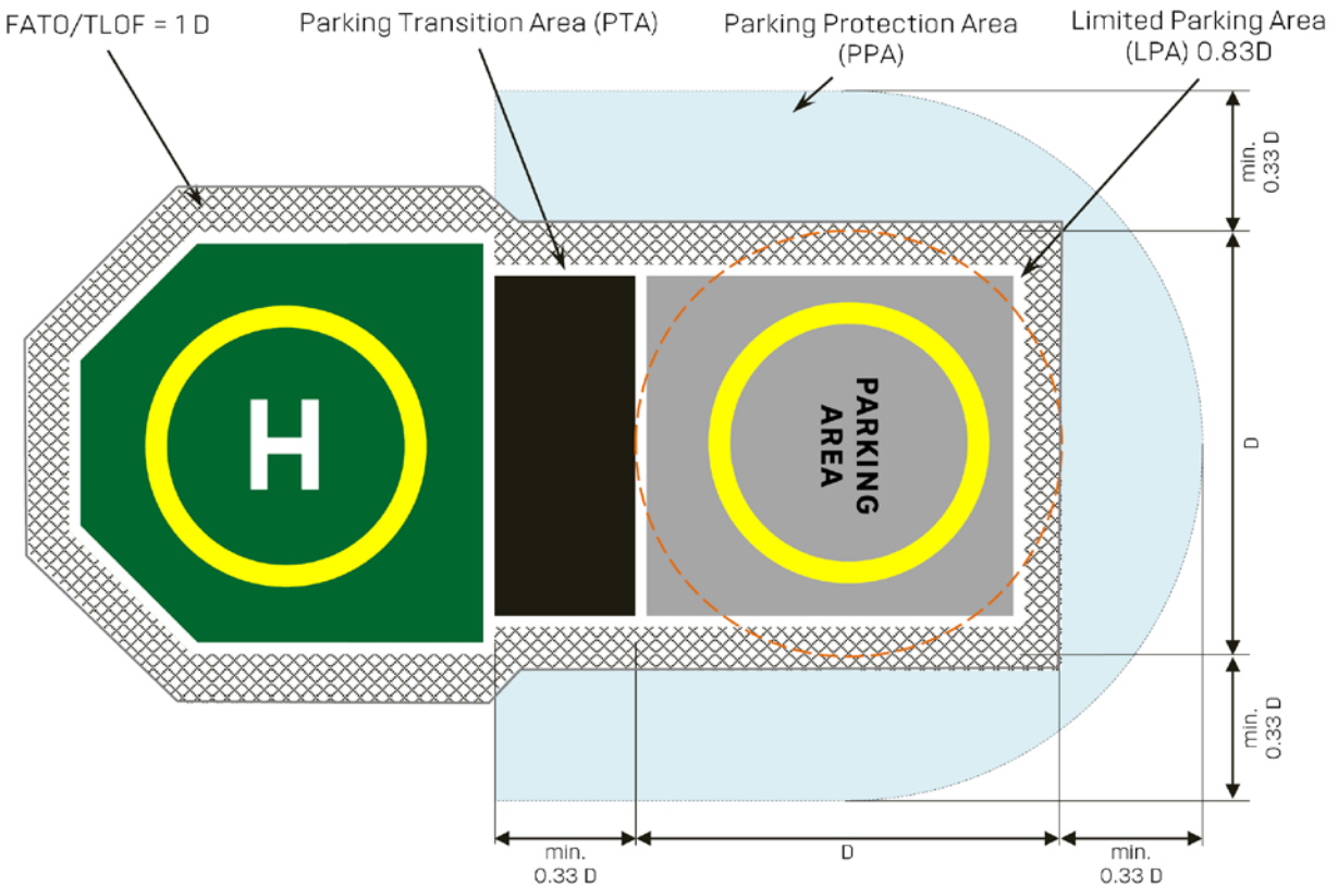
Figure 39: 1.0D FATO, 1.0D TLOF, and Limited Parking Area of 0.83D (RD)
