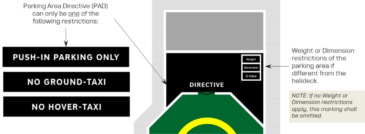
Figure 51: Parking Transition Area (PTA) associated markings
