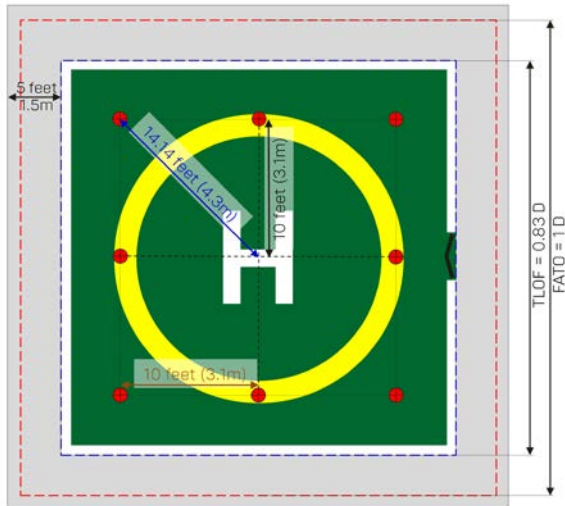
Figure 55: Tie-down point arrangement for an offshore-based helicopter on 0.83D TLOF helideck (a)
