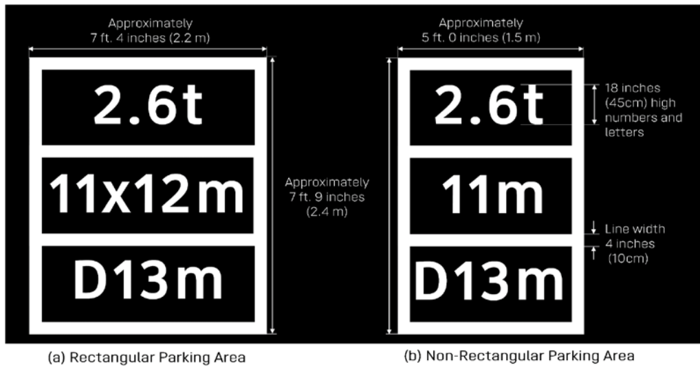
Figure 53: Metric Parking Area size/weight markings
