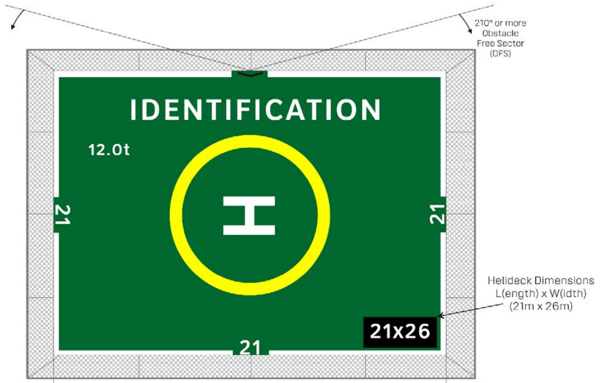
Figure 24: Size and weight markings for SI units
