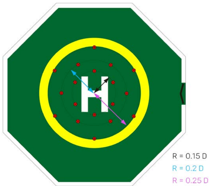
Figure 15: Tie down point arrangement
