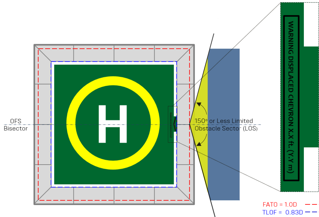
Figure 25: Example of a 0.1D displaced TDPM and 'H' for a helideck with 0.83D TLOF and 1.0D FATO
