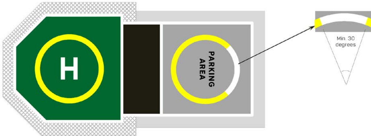
Figure 40: Touchdown Parking Circle (TDPC) marking and Parking Circle Orientation Marking (PCOM)
