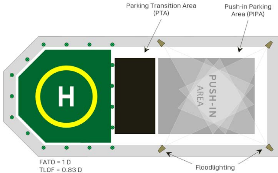
Figure 54: Push-in Parking Area (PIPA) lighting arrangement
