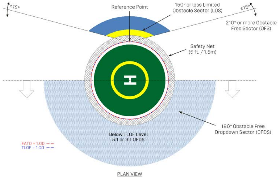
Figure 10: OFS, LOS, and OFDS below a helideck with 1.0D circular TLOF
