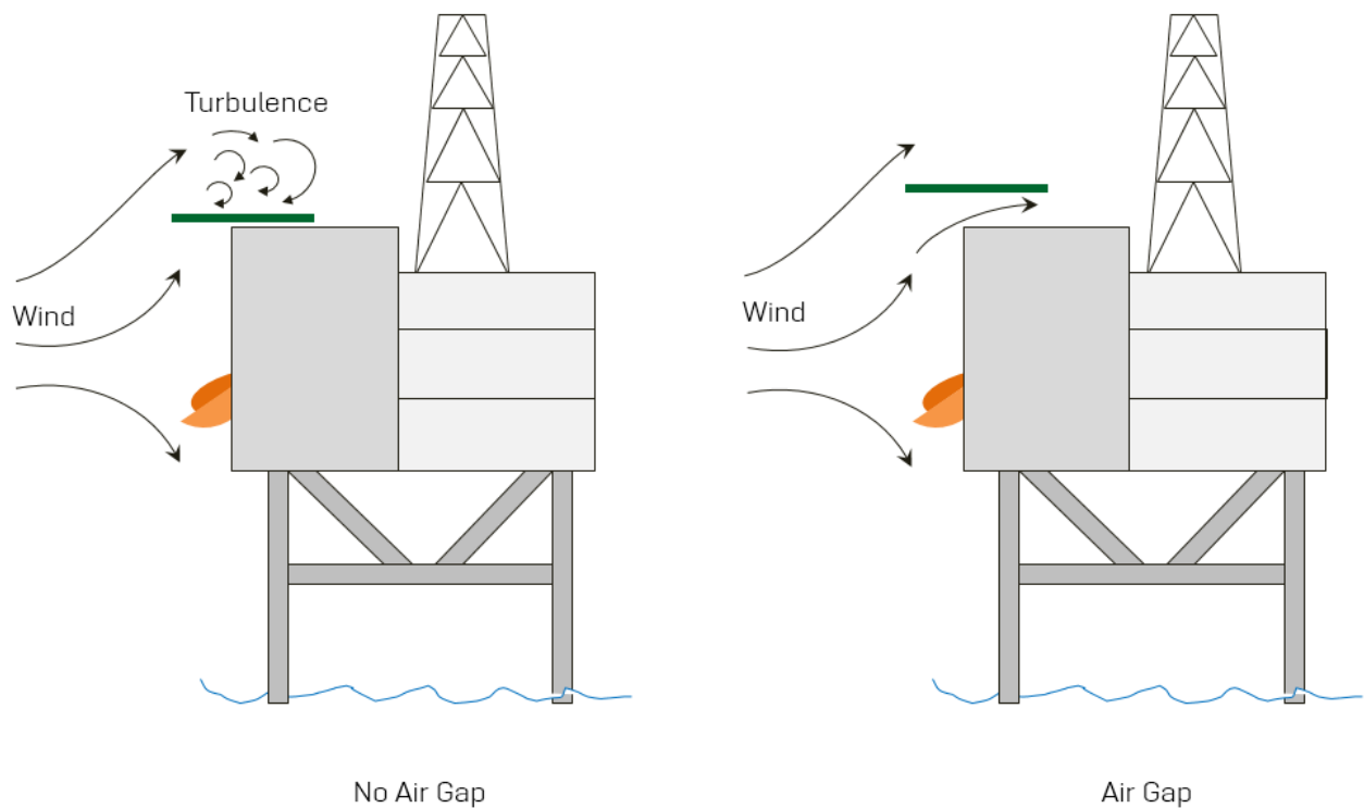
Figure 5: Turbulence with and without a Helideck Air Gap
