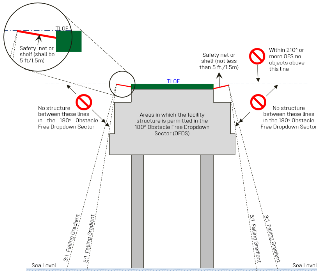
Figure 3: Illustration of OFDS
