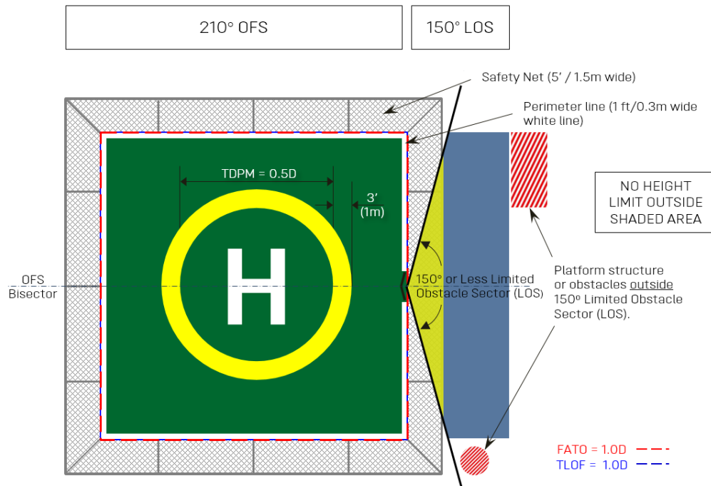
Figure 2: Illustration of OFS and LOS
