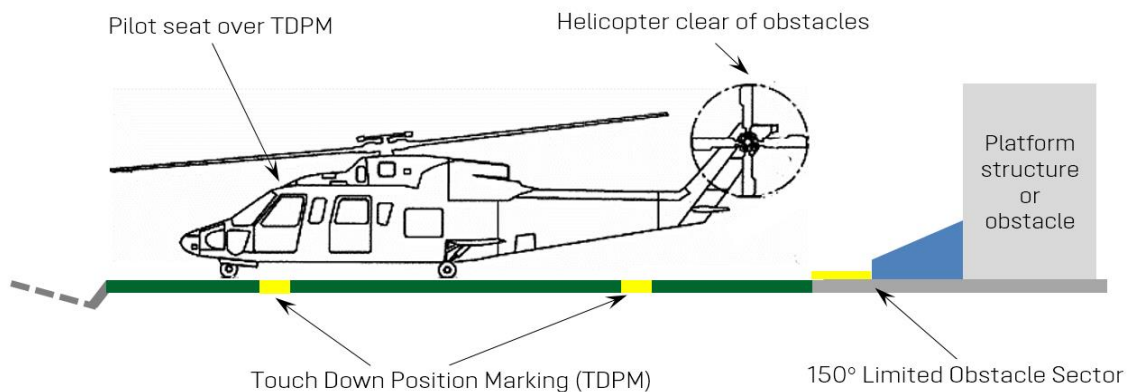
Figure 7: Relationship of the TDPM to LOS for a 1.0D TLOF
