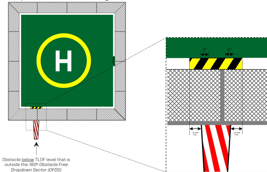
Figure 8: Obstacle Warning Marking for OFDS
