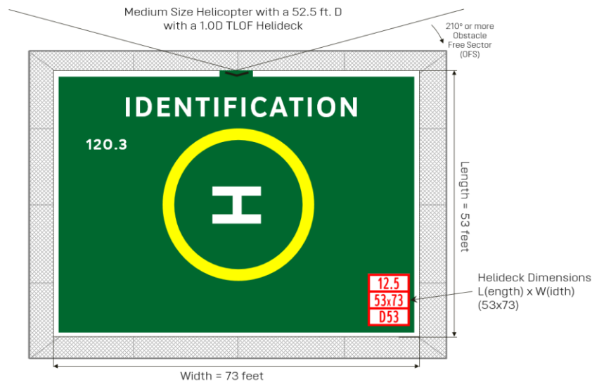
Figure 6: Typical Markings for 1.0D 52.5 ft. Medium Helicopter Rectangular Helideck
