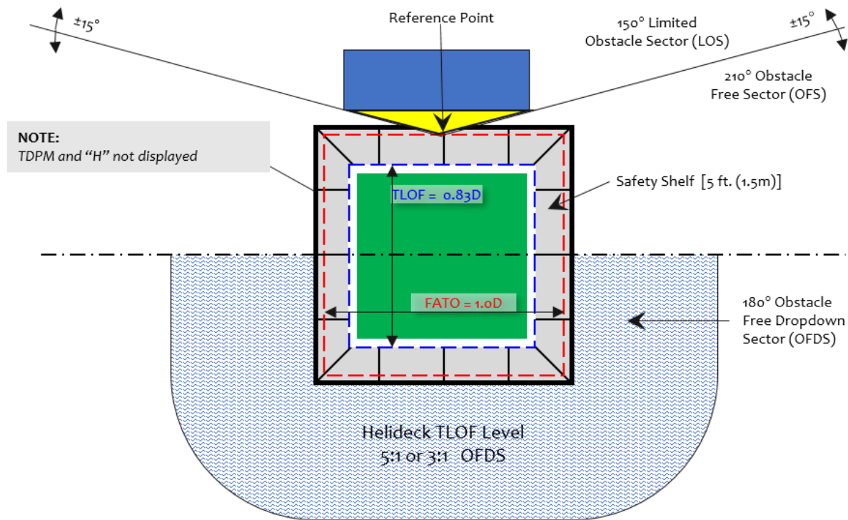
Figure 3.4.4.A Obstacle Free Sector, Limited Obstacle Sector and Obstacle Free Dropdown Sector for Helideck with 0.83D TLOF
