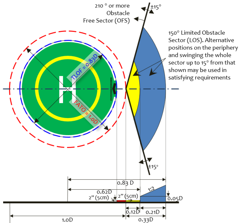
Figure 3.4.1.B Obstacle Limitation Sector and Obstacle-Free Sector for a Helideck with a Circular 1.0D FATO and 0.83D Circular TLOF
