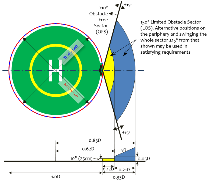
Figure 3.4.1.A Obstacle Limitation Sector and Obstacle-free Sector for a Helideck with a Circular 1.0D FATO and 1.0D Circular TLOF
