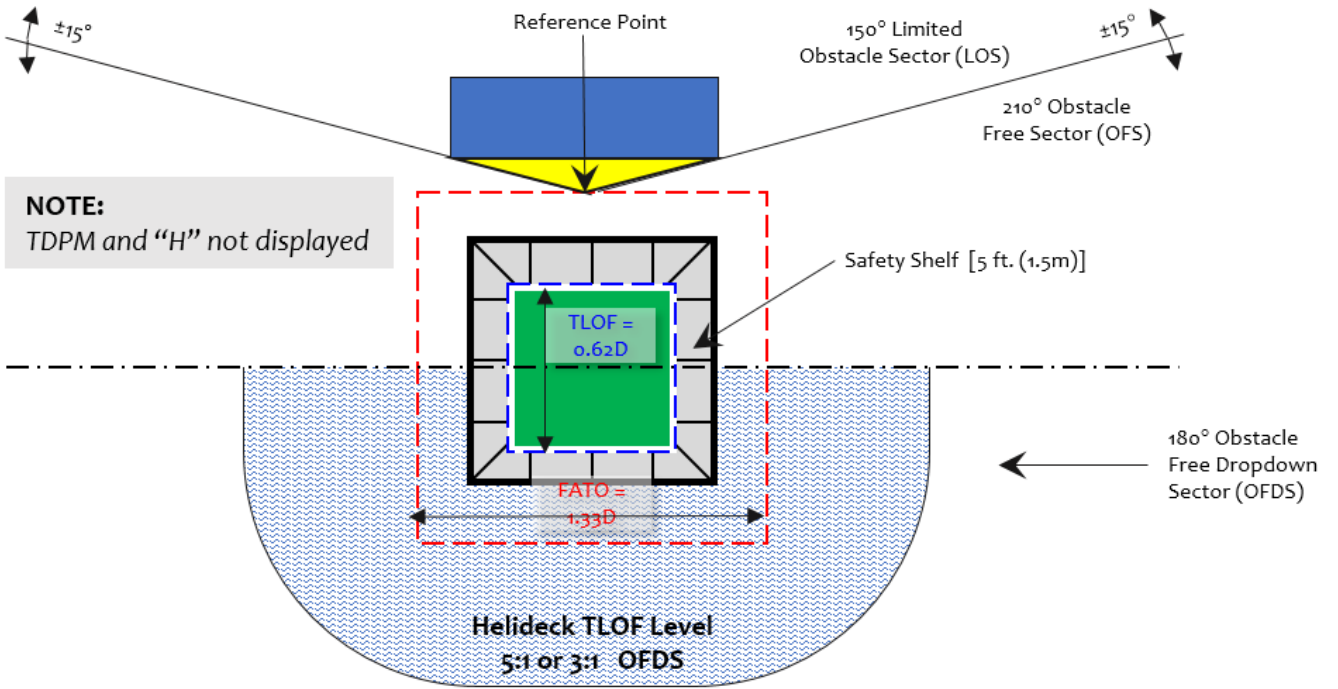
Figure 3.4.4.B Obstacle Free Sector, Limited Obstacle Sector and Obstacle Free Dropdown Sector for Helideck with 0.62D TLOF
