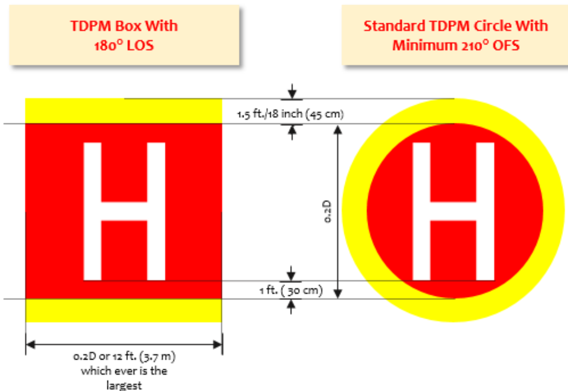
Figure 4.3.1.B. TDPM and H Marking for a Helidecks with a 0.62D to less than 0.83D TLOF
