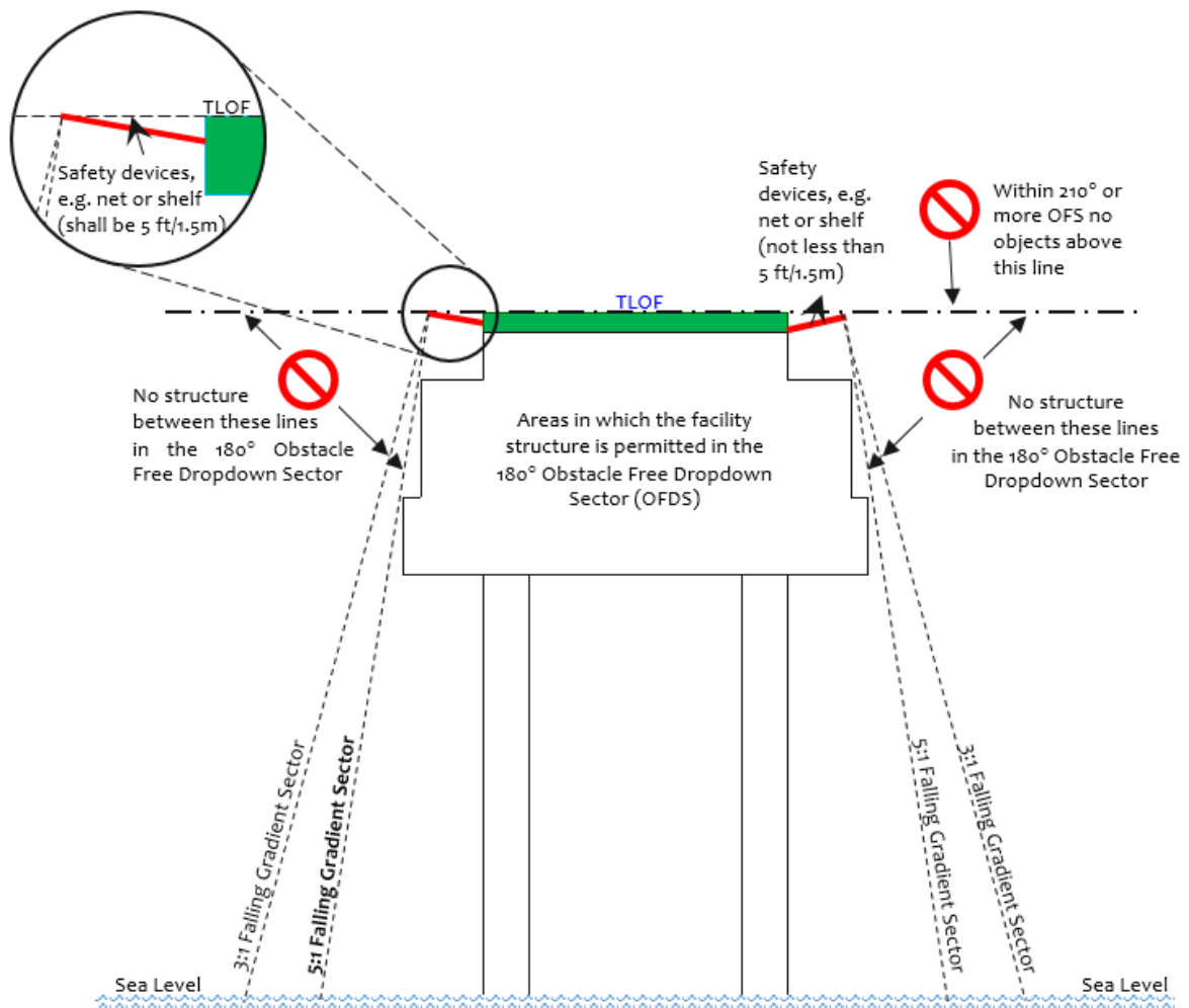
Figure 3.4.4.C Obstacle Free Sector (OFS) and Obstacle Free Dropdown Sector (OFDS)
