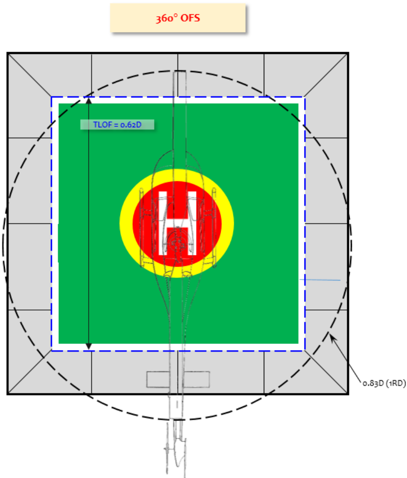
Figure 4.3.1.D TDPM for 0.62D TLOF with a 360° OFS
