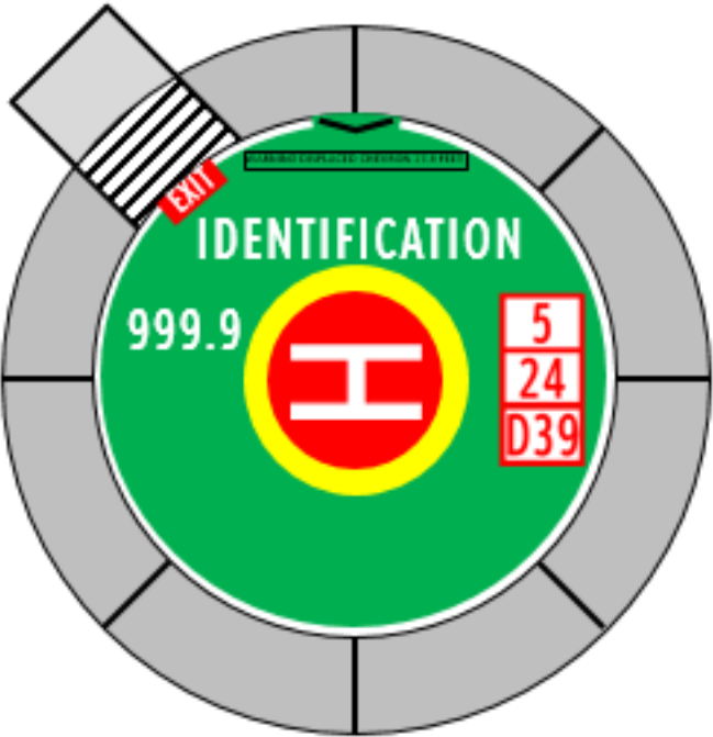
Figure 4.5D D-value, TLOF Size and Weight Markings for a 0.62D TLOF with a Circular TLOF
