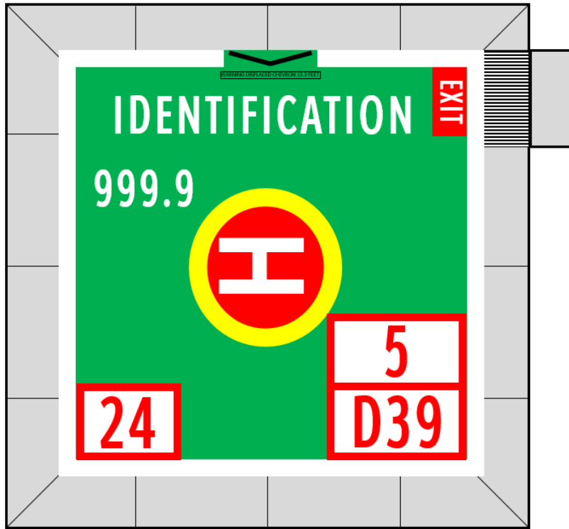
Figure 4.5.A D-value, TLOF Size and Weight Markings for a Square 0.62D TLOF (i.e medium size twin engine transport helicopter, like a Sikorsky S-76)
