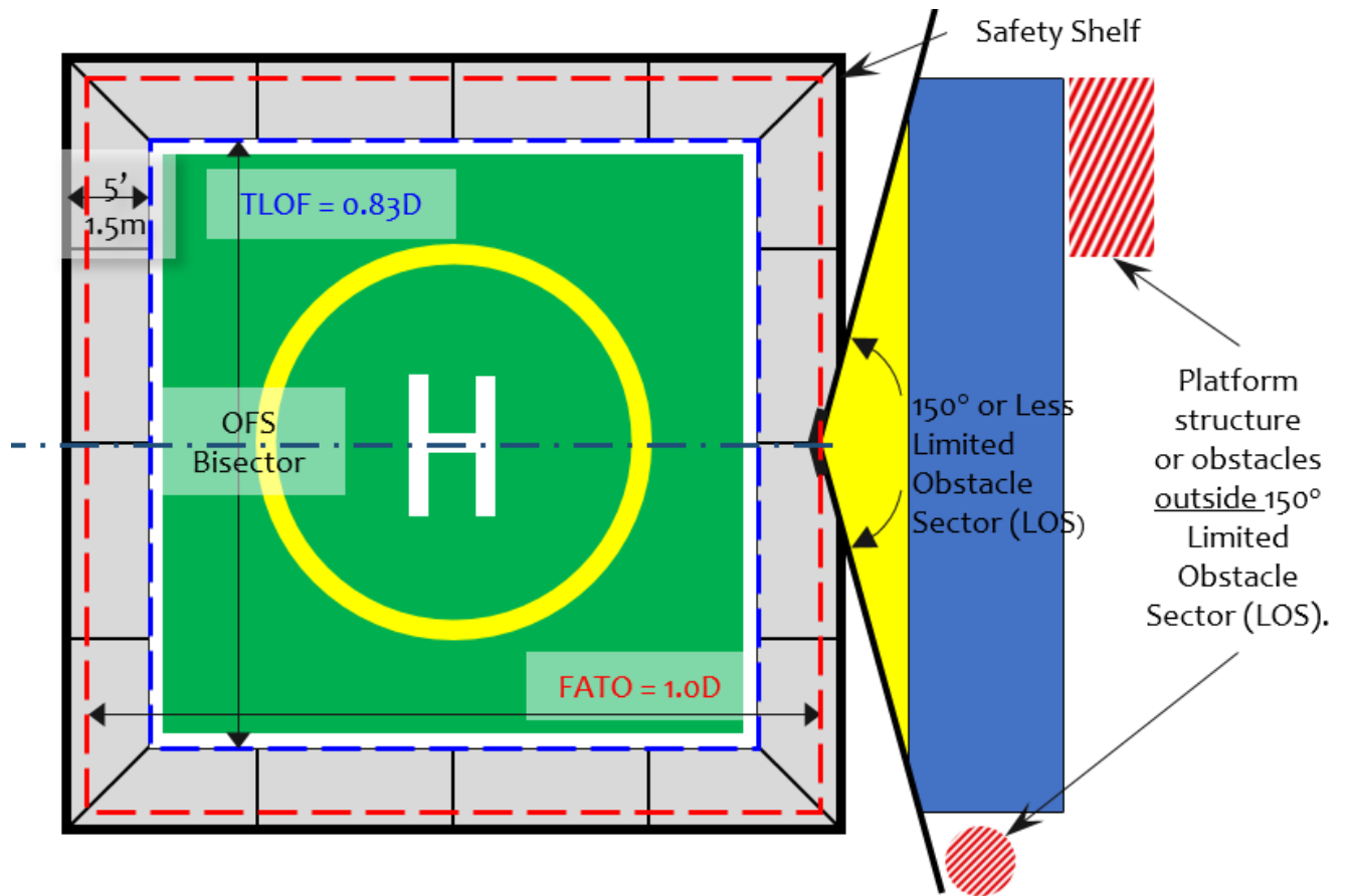
Figure 4.6.1.B Chevron Marking for 0.83D TLOF on the Helideck Safety Shelf
