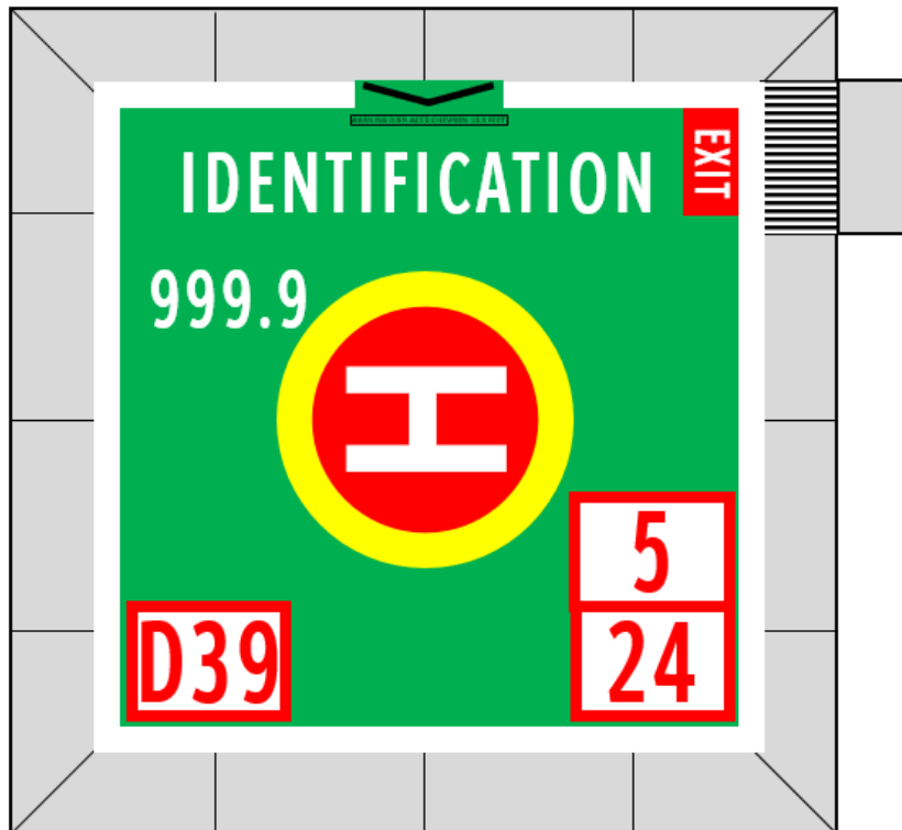
Figure 4.5.A D-value, TLOF Size and Weight Markings for a Square 0.62D TLOF (i.e medium size twin engine transport helicopter, like a Sikorsky S-76)
