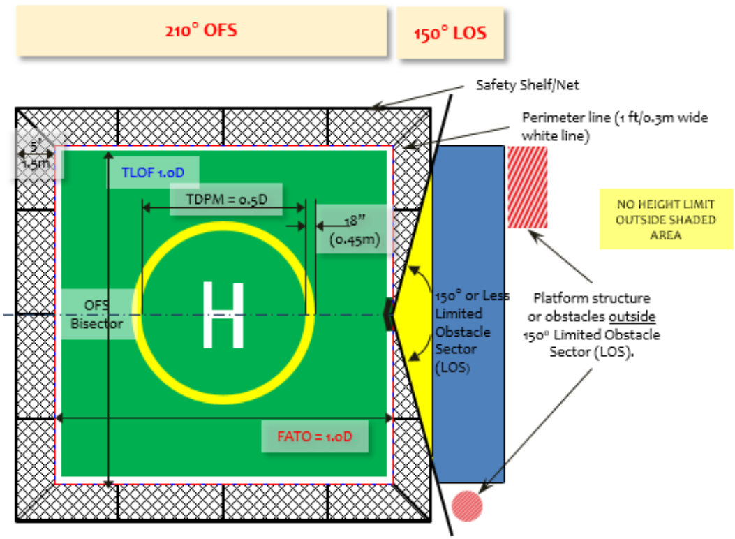
Figure 3.3.1.A Square Helideck with a 1.0D FATO, a 1.0D TLOF and a 210° OFS / 150° LOS
