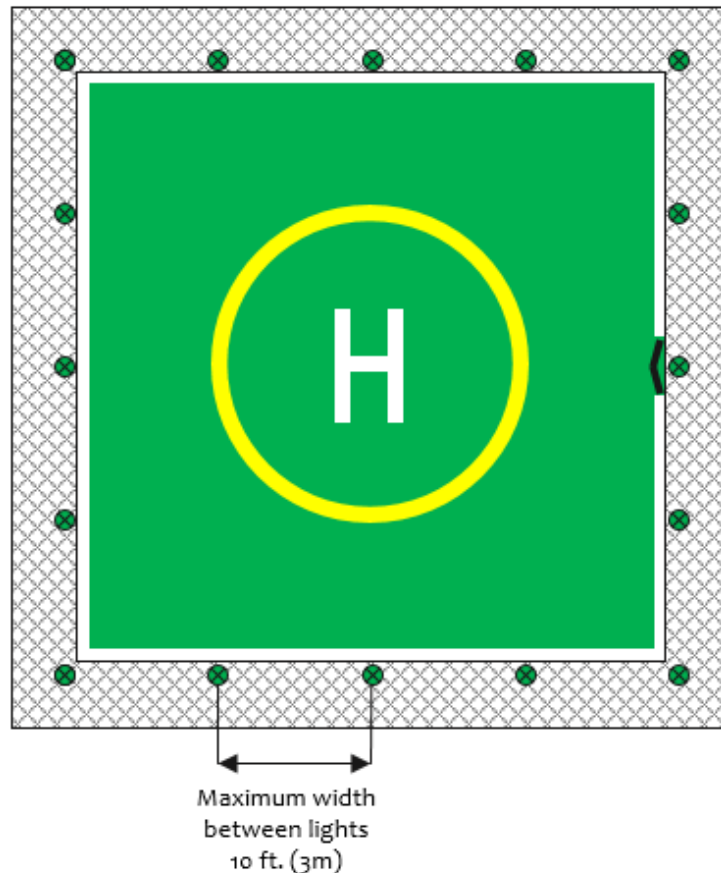
Figure 5.1 Example of Typical TLOF Lighting Arrangement for a 0.83D TLOF
