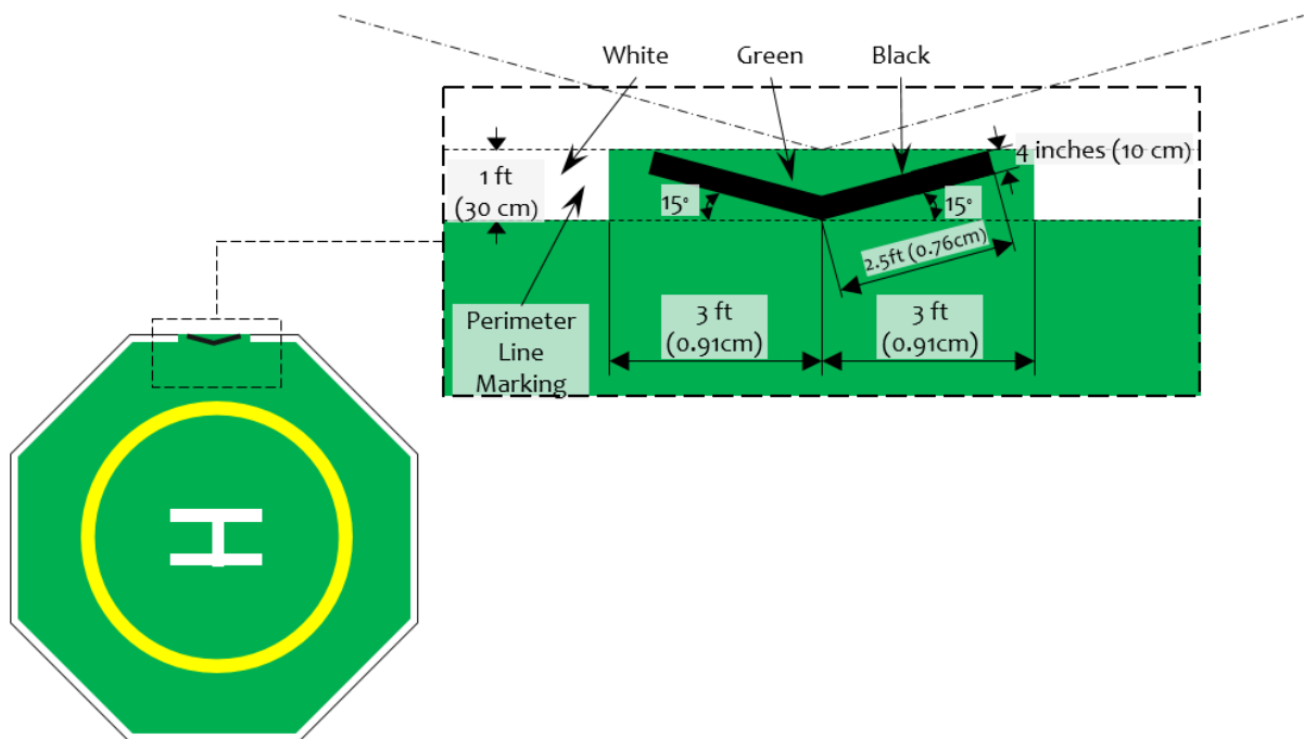
Figure 4.6.1.A Standard Chevron Marking
