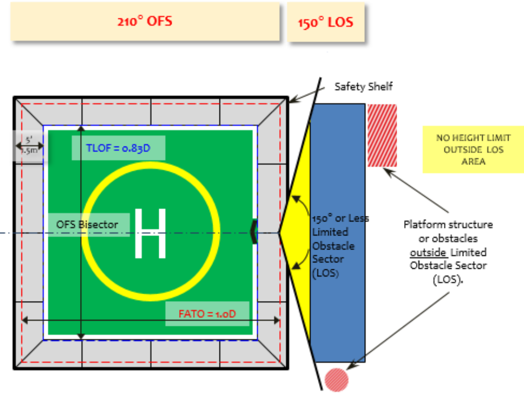
Figure 3.3.1.B Square Helideck with 1.0D FATO, a 0.83D TLOF and an OFS of 210°
