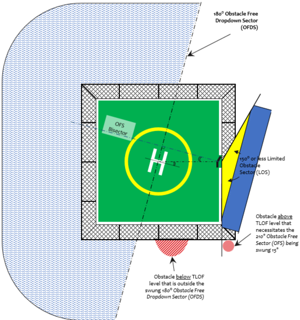
Figure 3.4.5 OFS Sector Swung by 15°
