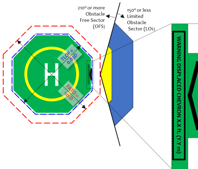
Figure 4.6.2.A Displaced Chevron Marking
