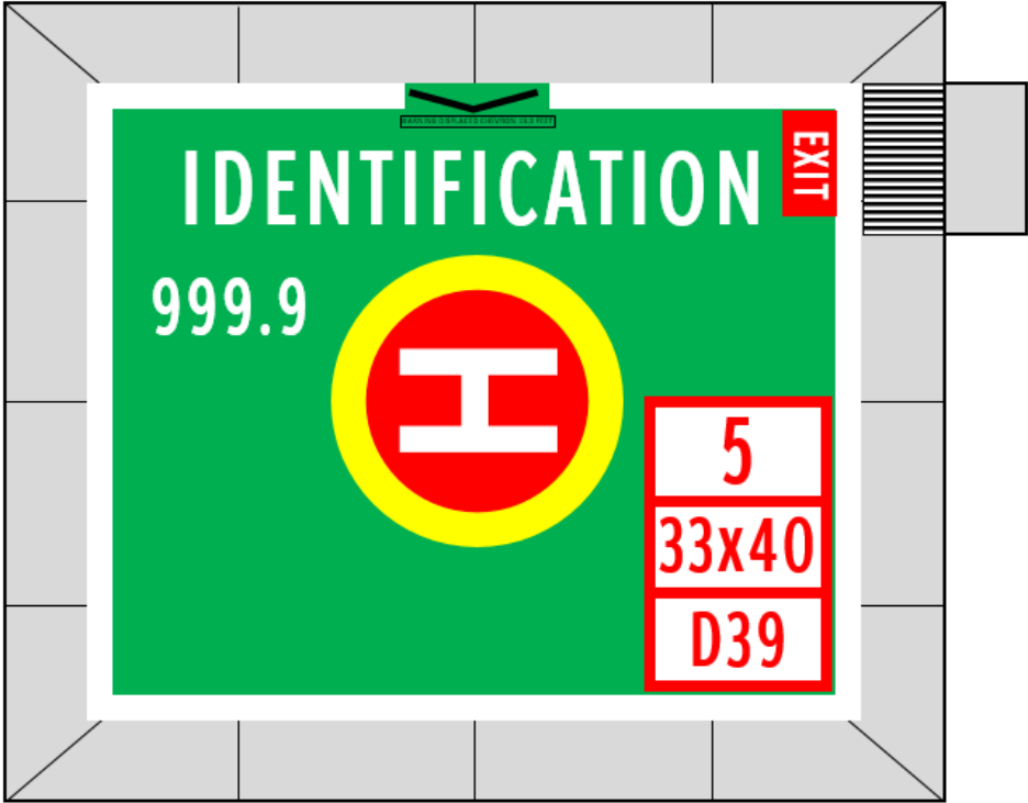
Figure 4.5.C D-value, TLOF Size and Weight Markings for a 0.62D a Rectangular TLOF (ie. single engine helicopter, like a Bell 206)
