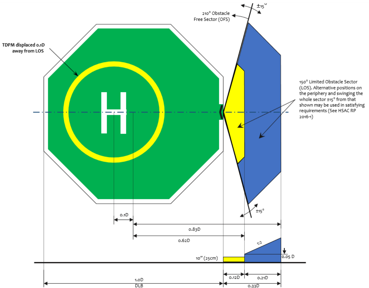
Figure 4.3.1.A. Displaced TDPM for a TLOF a 1.0D TLOF
